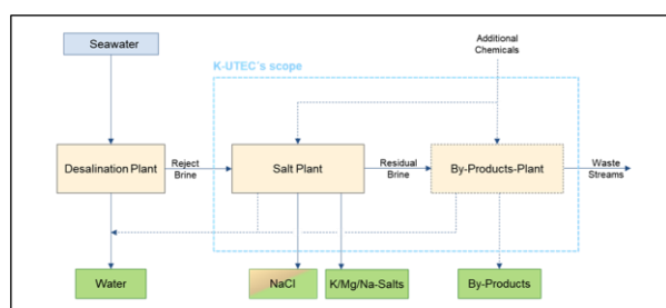
Fig. 2: General flow chart of the project (K-UTEC). N.b. although the project's scope is focused on salt recovery and by-products, the necessary analysis and linkages with the green hydrogen industry and desalination plants will be established, such as heat integration analysis and benefits for green hydrogen production costs.
